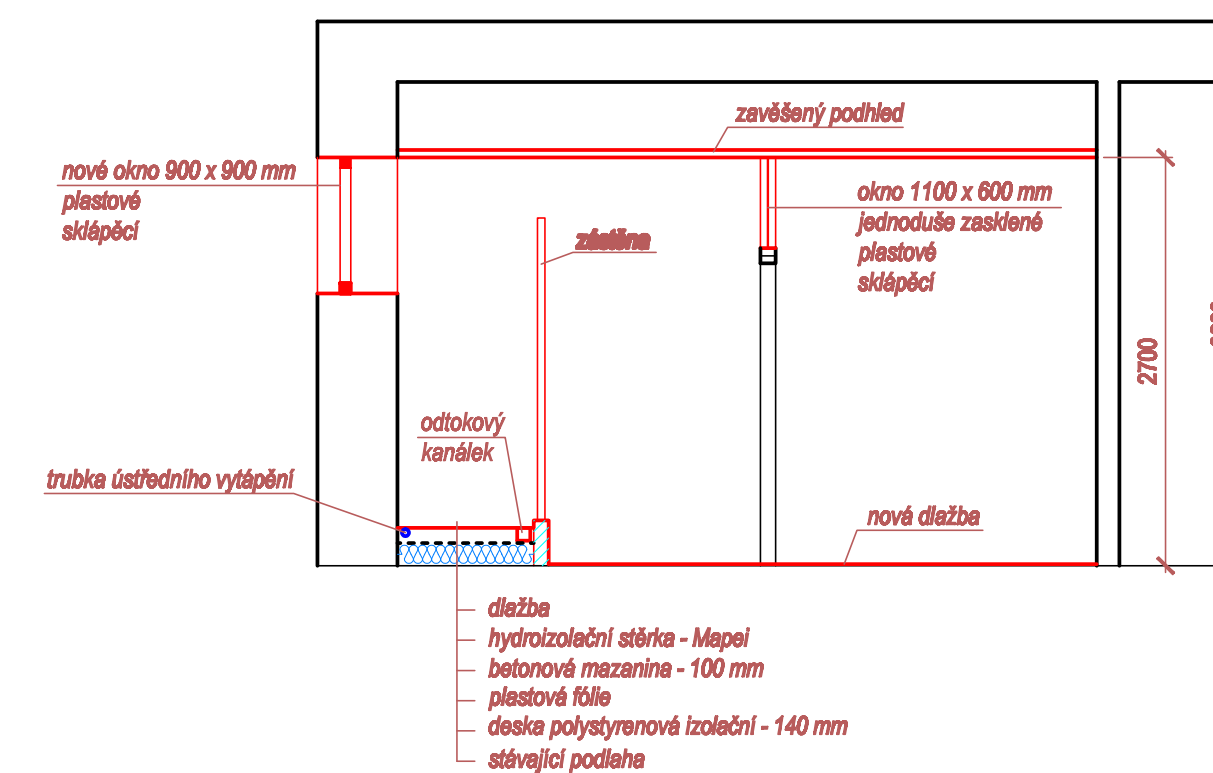
DETAIL B
